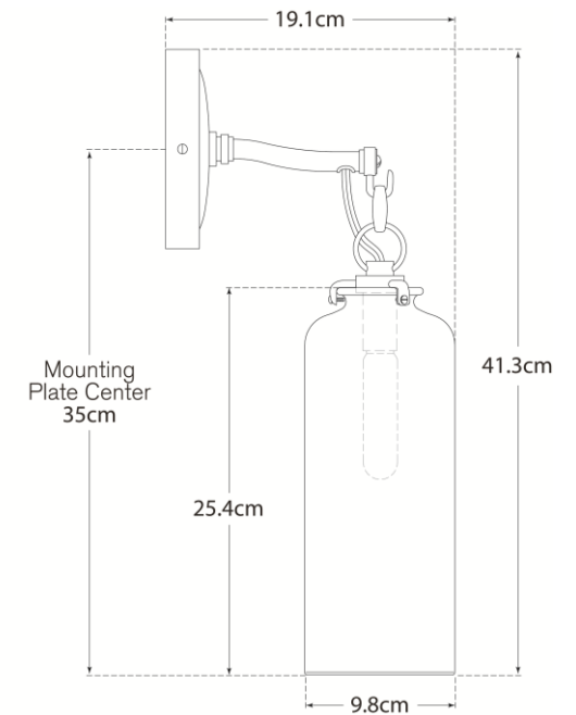
Front View Mounting Plate
